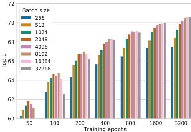
Figure B.2. Linear evaluation (top-1) of ResNet-50 trained with different batch sizes and longer epochs. Here a square root learning rate, instead of a linear one, is utilized.
